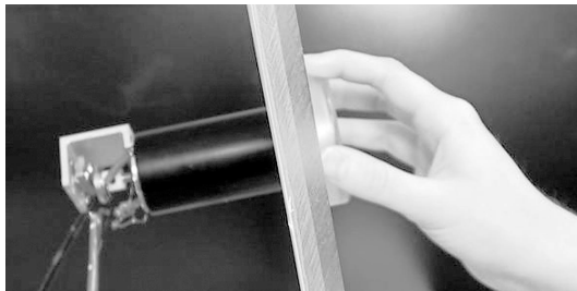
Figure 5.5. A force feedback knob. A computer algorithm takes sensed knob position as input into a virtual model and produces an output torque, which is delivered through the knob's motor. Photo used with permission of Colin Swindells.
